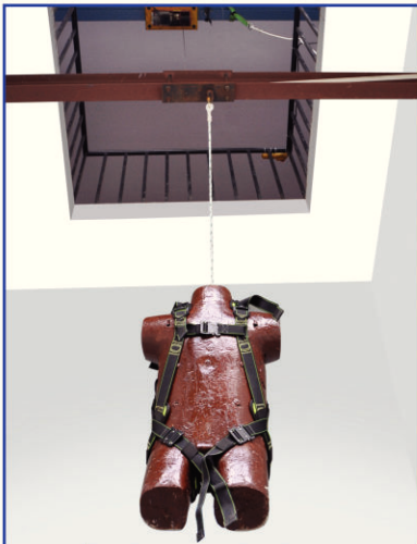
Dynamic Performance Testing
