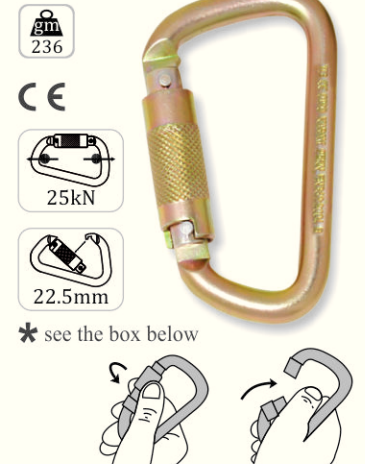
Ref. PN 113 Steel Quarter Turn-Locking Karabiner
