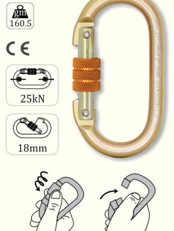
Ref. PN 112 Steel Screw-Locking Karabiner
