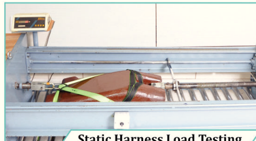
Static Harness Load Testing
